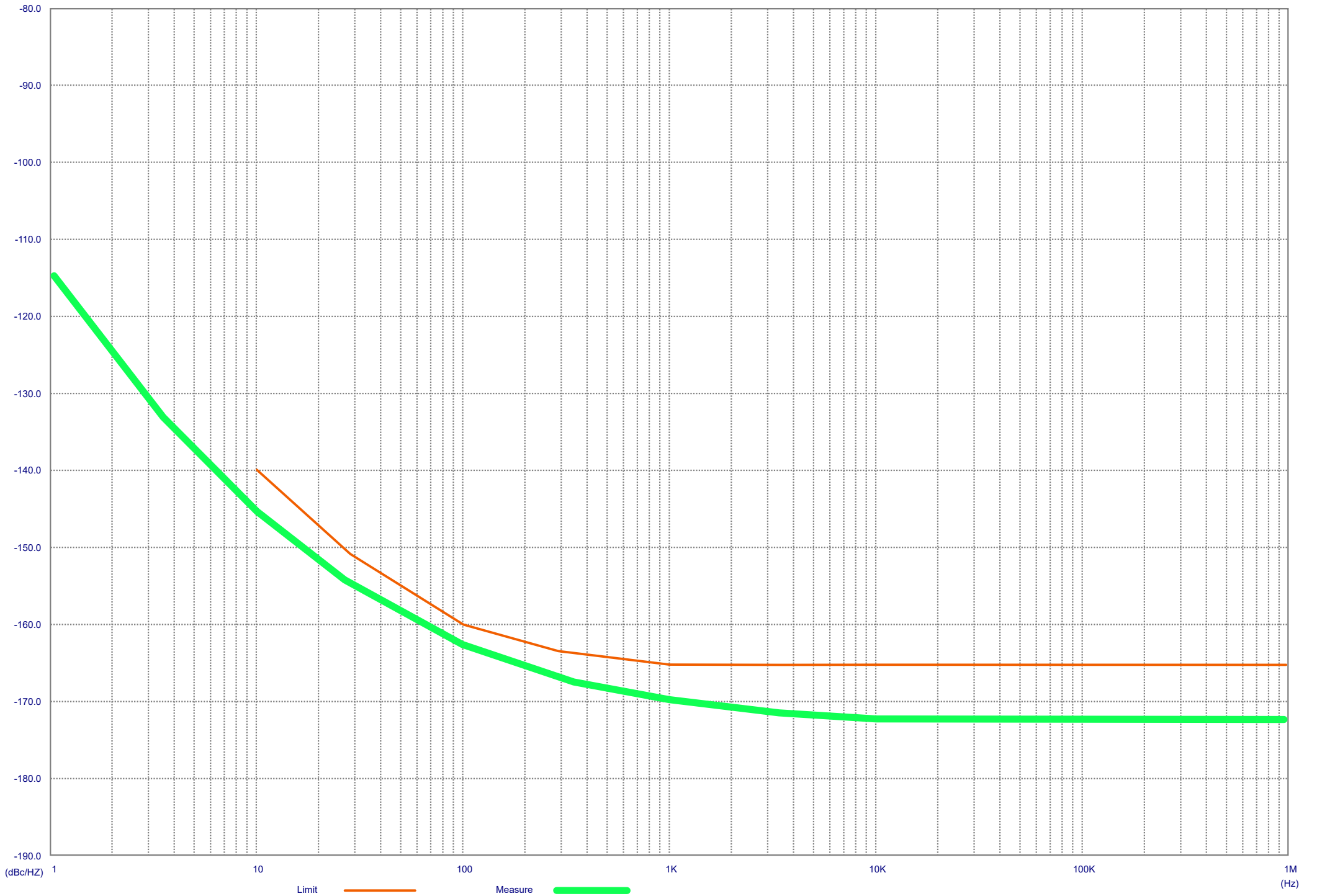
sCLK-OCX10 Phase noise graph
